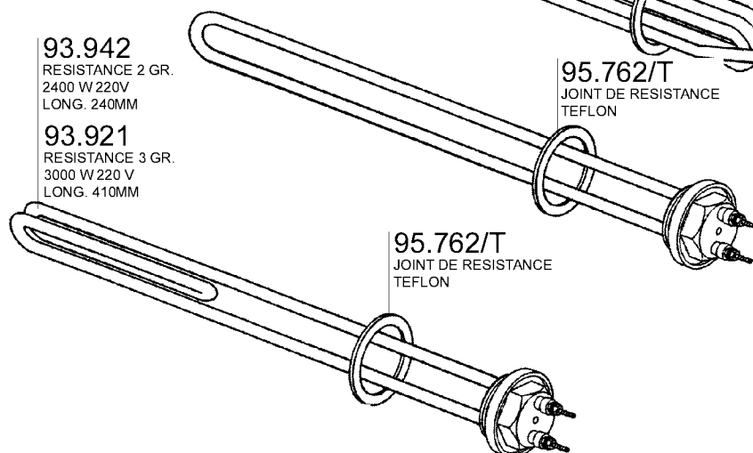
95.762/T JOINT DE RESISTANCE TEFLON
