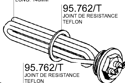
93.919 RESISTANCE 1 GR. 1500W 220V LONG. 140MM
