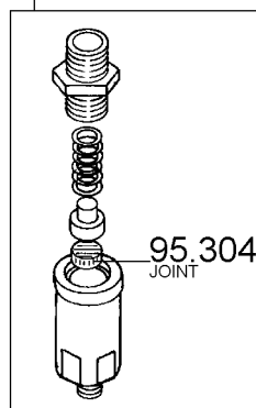
|93.767 SOUPAPE ANTI-RETOUR
