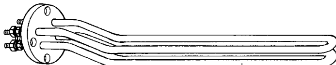
93.911 RESISTANCE 1 GR. 2000 W BEZZERA / VERA 93.912 RESISTANCE 2 GR. 2500 W VERA COMPACT 93.913 RESISTANCE 2 GR. 3500 W BEZZERA/ VERA
