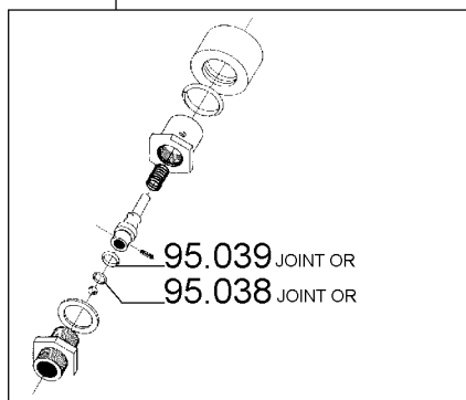
93.763 SOUPAPE DE SECURITE VERA
