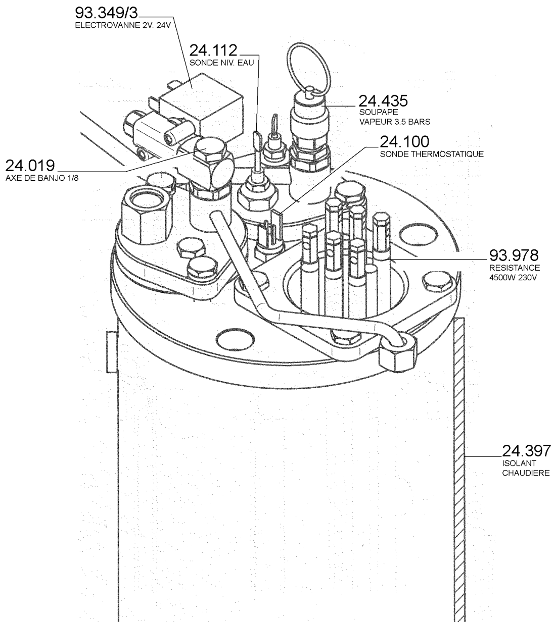
CHAUDIERE COMPLETE TANGO SOLO
