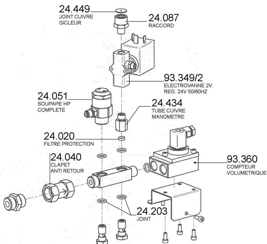
CHAUDIERE INTERNE TANGO SOLO
