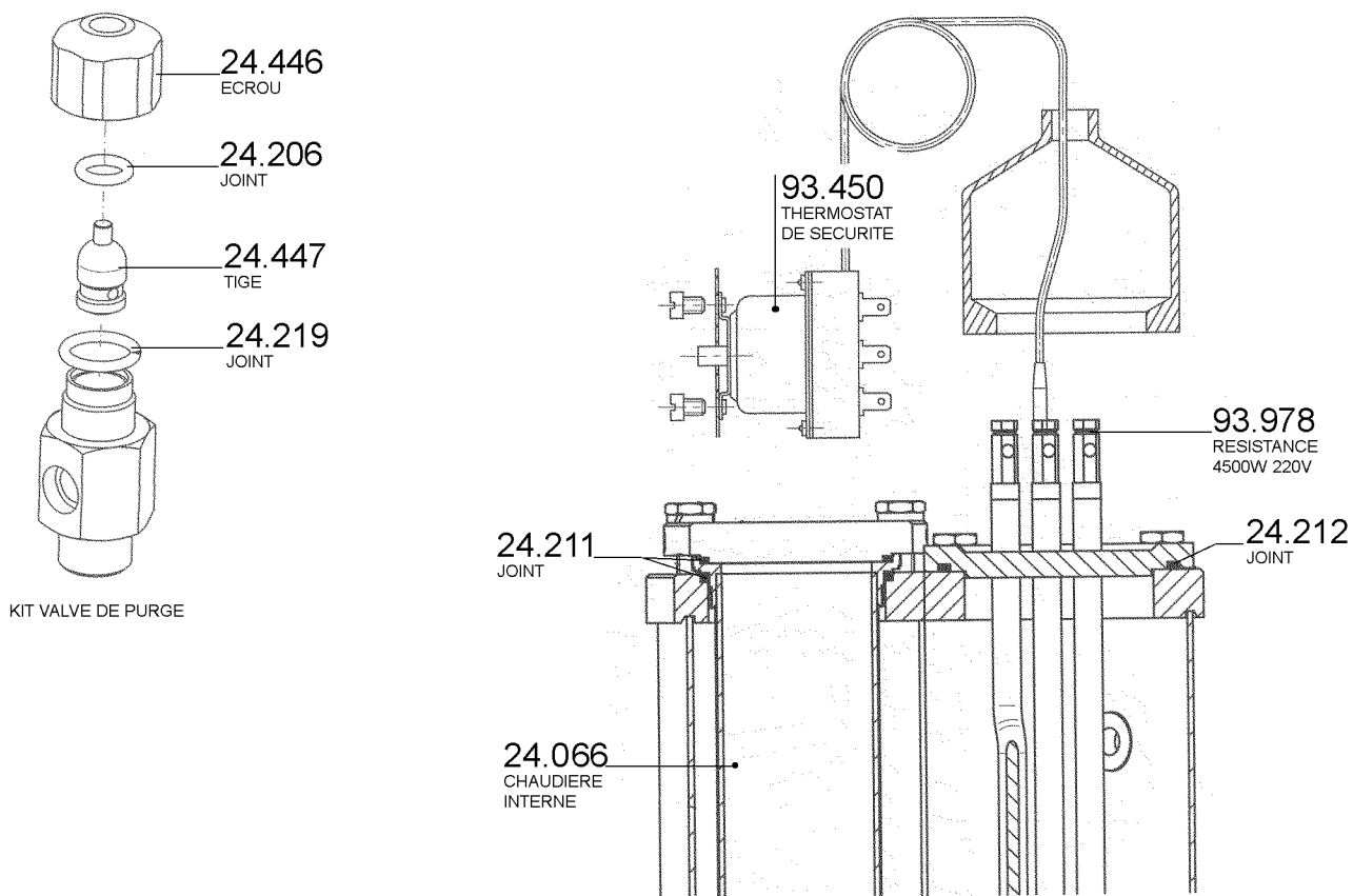
CHAUDIERE INTERNE TANGO SOLO
