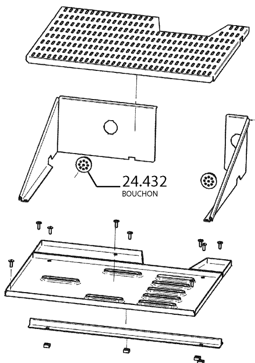
ENS. CHAUFFE TASSES TANGO 1 GR
