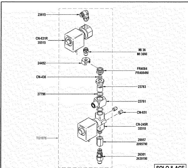
10/16 OPTION POMPE LAIT "VUE D'ENSEMBLE" "OVERVIEW" MILK PUMP KIT UNIC 600
