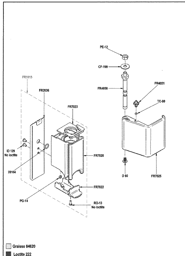
10/16 ENSEMBLE BEC & PORTILLON SET SPOUT & DOORS
