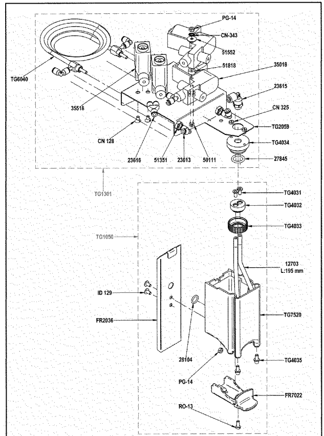
10/16 OPTION POMPE LAIT "BEC & BLOC LAIT" "SPOUT & MILK BLOCK" MILK PUMP KIT UNIC 601
