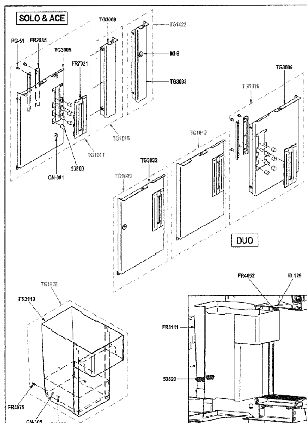
10/16 ENSEMBLE DEVANT & TIROIR A MARC SET WASTE DRAWER & FRONT CASING
