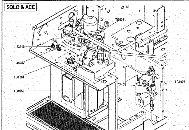
10/16 OPTION POMPE LAIT "VUE D'ENSEMBLE" "OVERVIEW" MILK PUMP KIT UNIC 600
