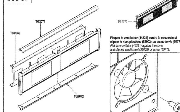
10/16 CALANDRE TANGO ST FRONT PANEL TANGO ST
