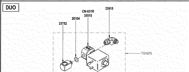
10/16 OPTION POMPE LAIT "ELECTROVANNES" "ELECTROVALVES" MILK PUMP KIT UNIC 602
