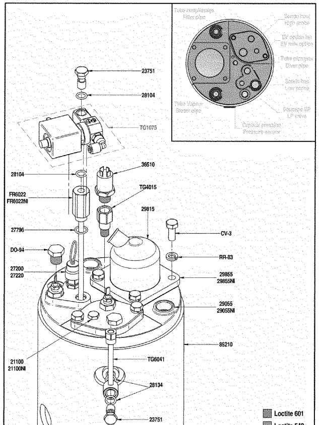
10/16 OPTION POMPE LAIT "CHAUDIERE DUO" "BOILER DUO" MILK PUMP KIT UNIC 604
